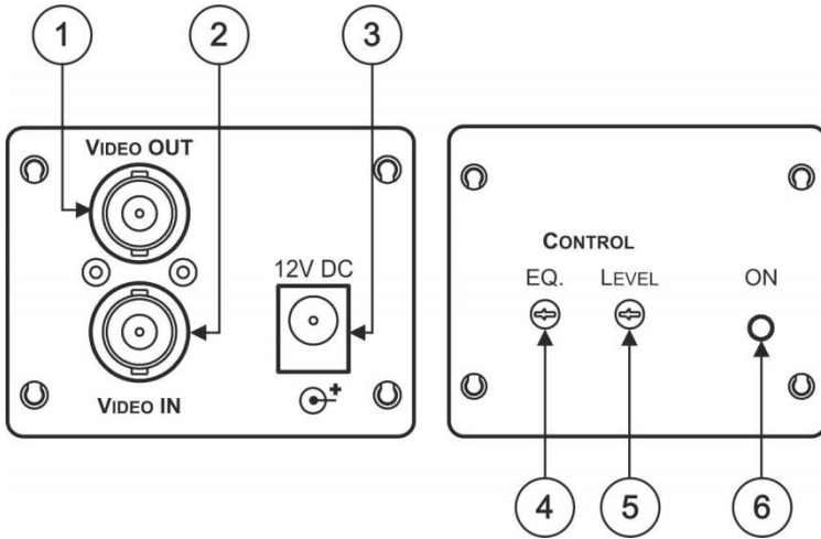
Figure 1: 101L Video Line Amplifier
